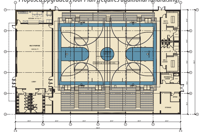
Proposed Upgraded Floor Plan (requires additional fundraising)
