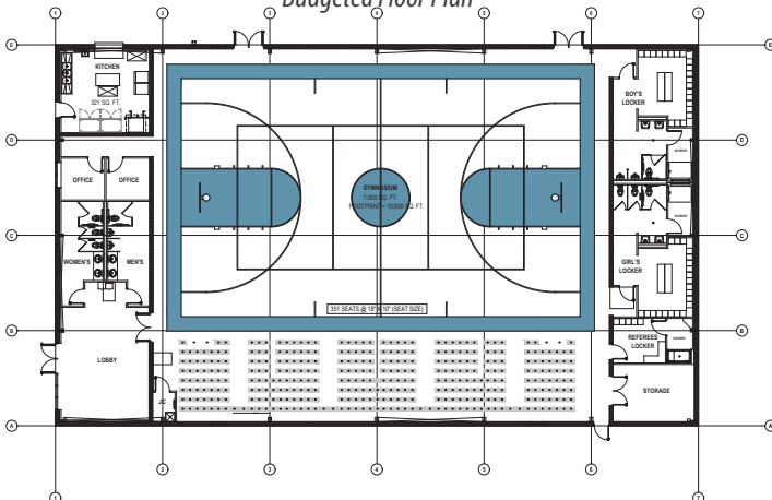
Budgeted Floor Plan
